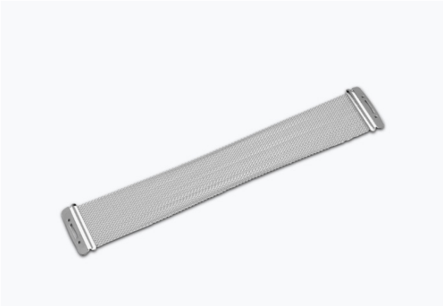
20-STRAND REPLACEMENT SNARE WIRES DSW1420 / 14261 Dimensions: 14" (L) Coils: Medium-gauge 0.6 mm Construction: 20-strand steel wires / chrome-plated end clips
